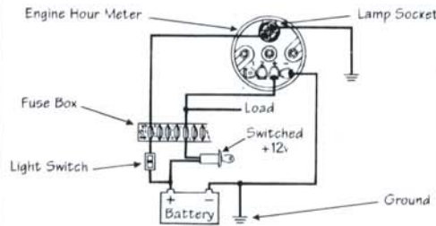
Proper wiring of Engine Hourmeter
