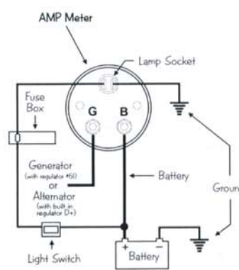
Proper wiring of AMP Meter
