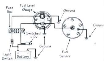
Proper wiring of Fuel Gauge
