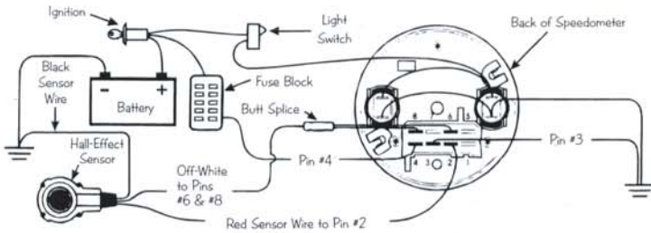
Proper wiring of Speedometer using: Hall-Effect Sensors
