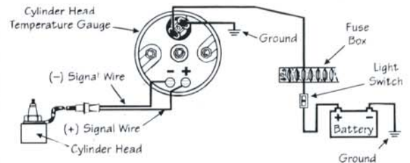
Proper wiring of the Cylinder Head Temperature Gauge
