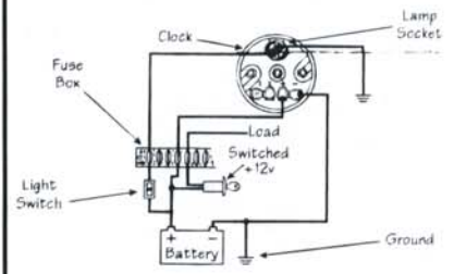
Proper wiring of Quartz Clock
