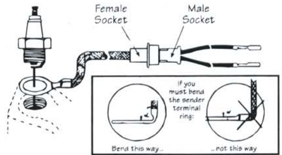
Proper installation of the Cylinder Head Temperature Sender
